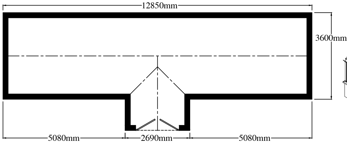
FLOOR PLAN
